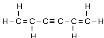
Structure 2
