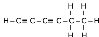
Structure 3
