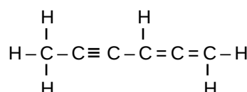
Structure 6
