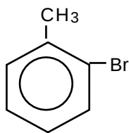
o-bromotoluene
