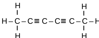
Structure 4
